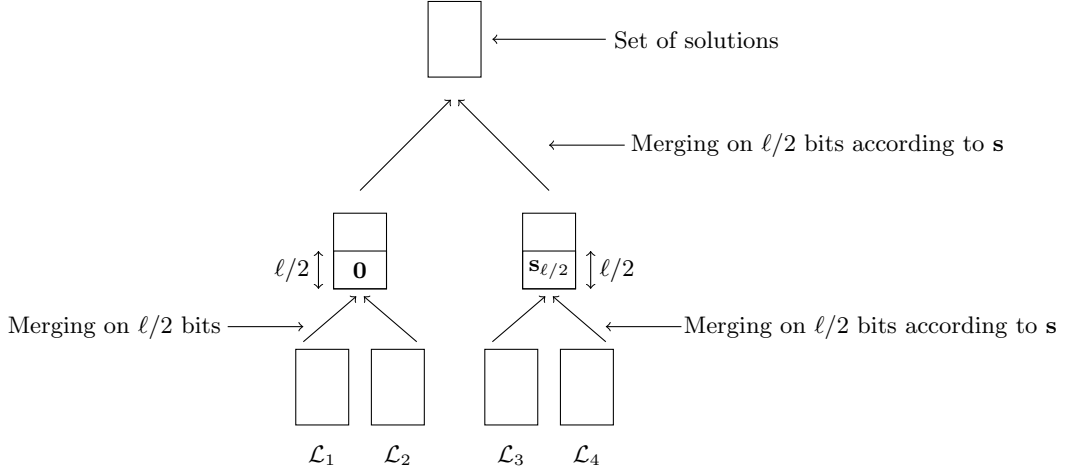
Fig. 2. Wagner's algorithm with a = 2 .
