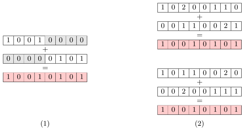
Fig. 3. Same vector (1) using left-right split and (2) using representations.
